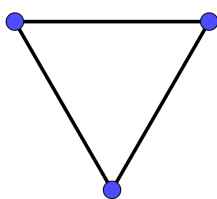
Obr. 3.9: Graf K_3
